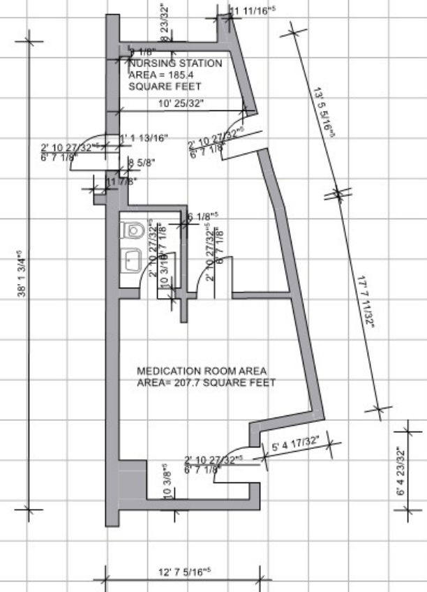
NEW NURSING STATION FLOOR PLAN
