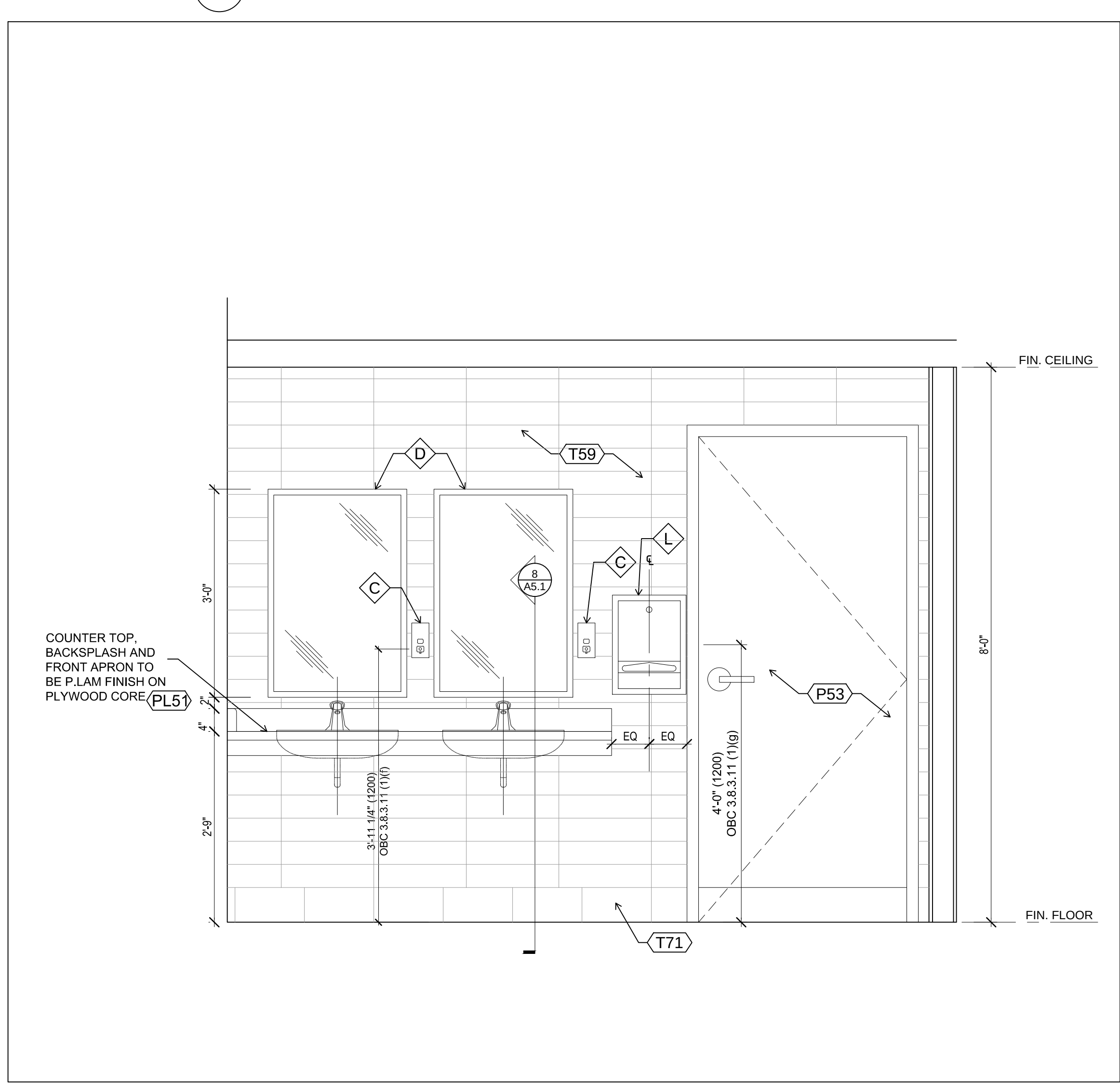
13 WOMENS WASHROOM - EAST ELEVATION SCALE: 3/4"=1'-0"
