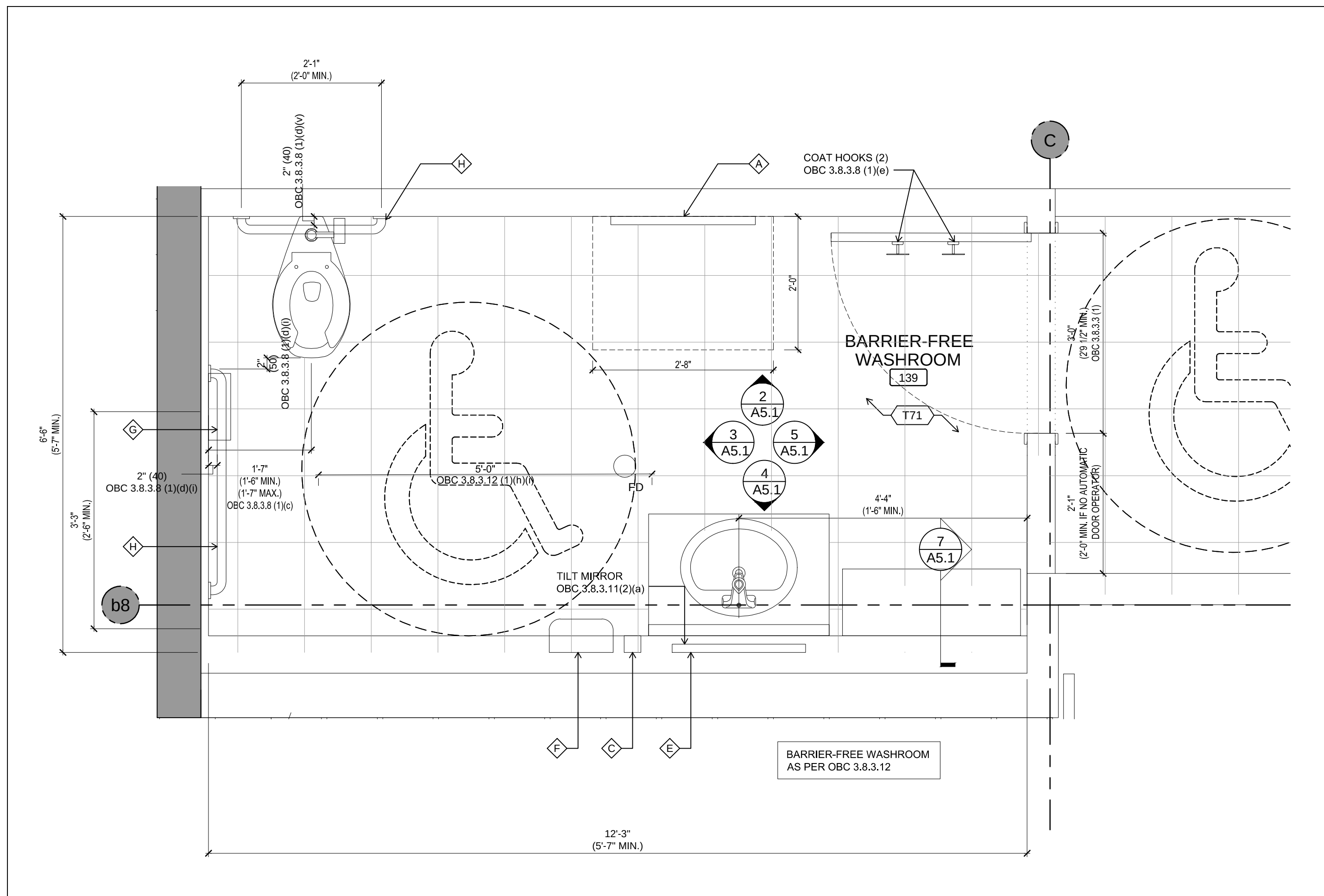
1 BARRIER-FREE WASHROOM SCALE: 3/4"=1'-0"
