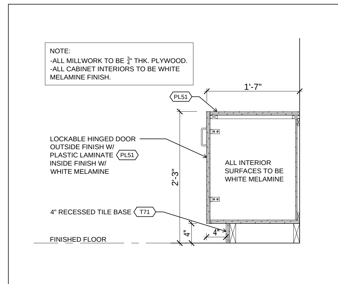
7 WASHROOM CABINET SECTION SCALE: 1/2"=1'-0"
