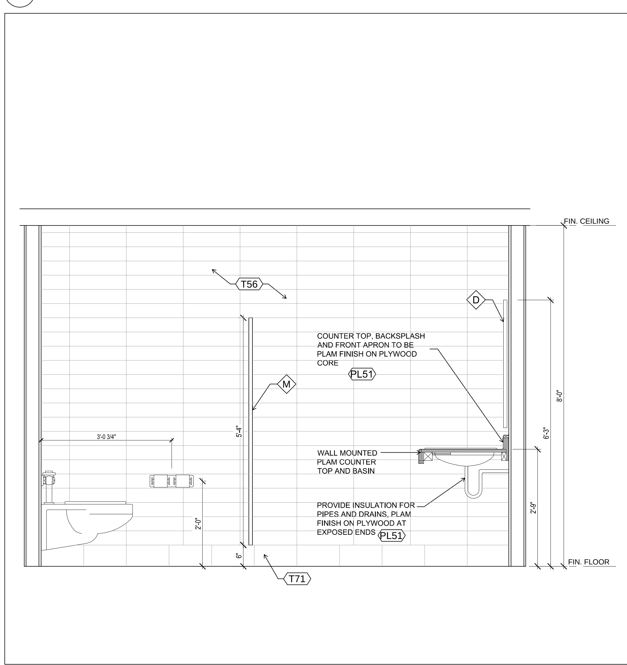
12 WOMENS WASHROOM - NORTH ELEVATION SCALE: 3/4"=1'-0"
