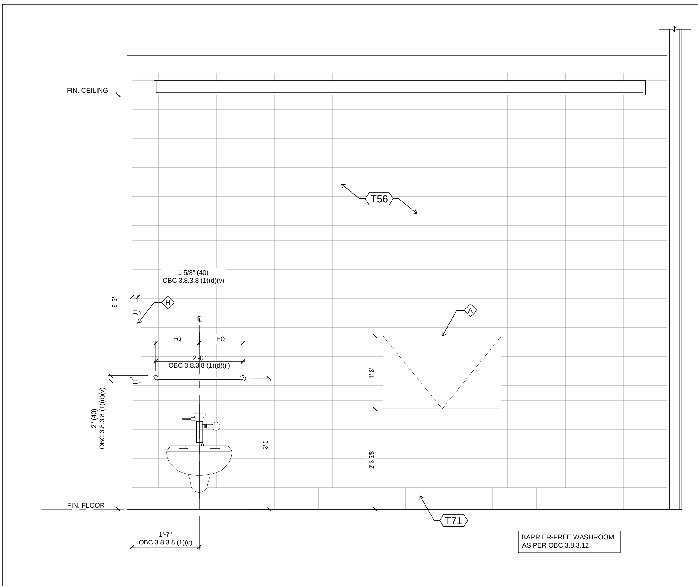
2 BARRIER-FREE WASHROOM - NORTH ELEVATION SCALE: 3/4"=1'-0"
