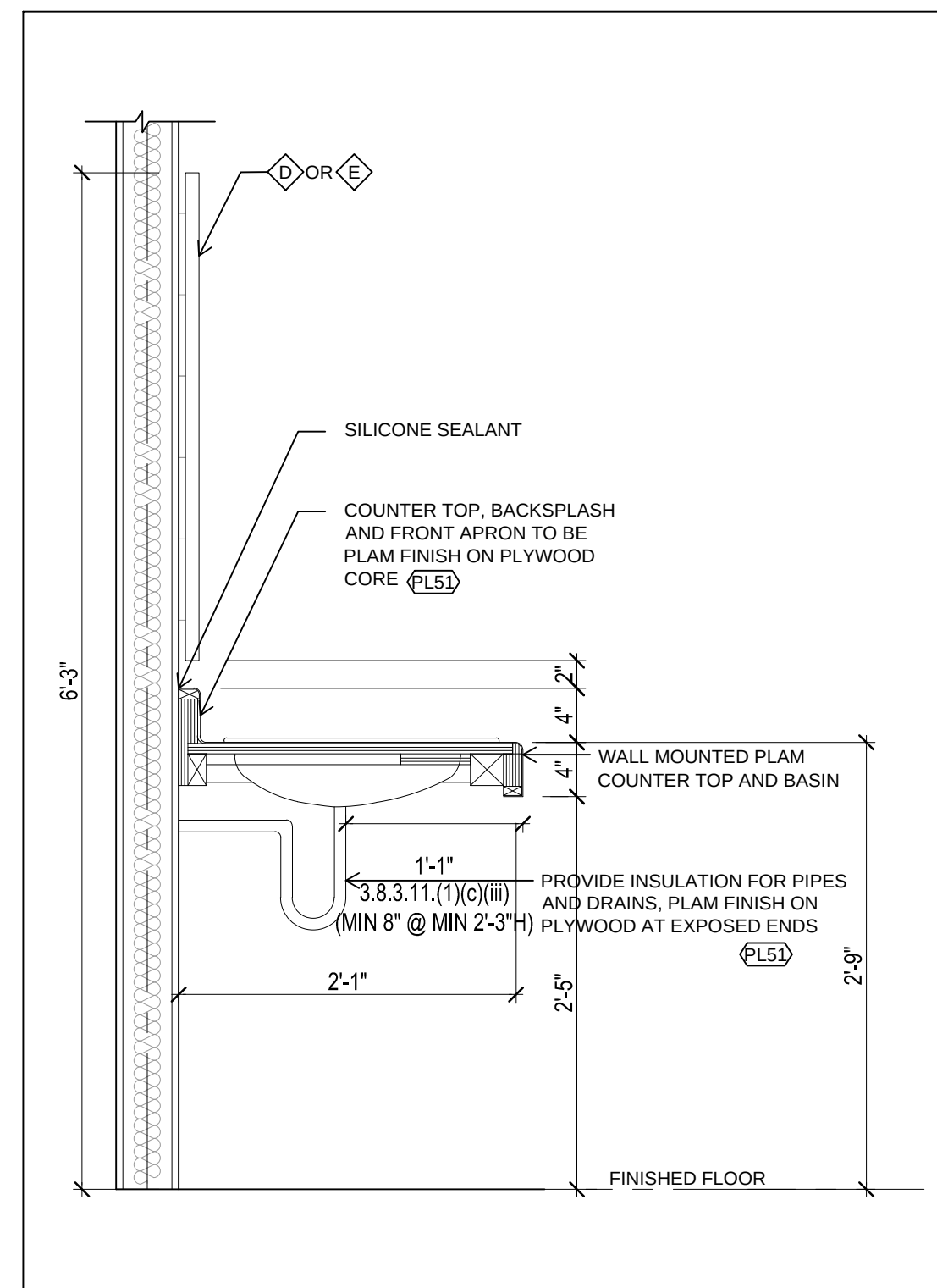
8 STAFF WASHROOM SINK DETAIL SCALE: 1/2"=1'-0"
