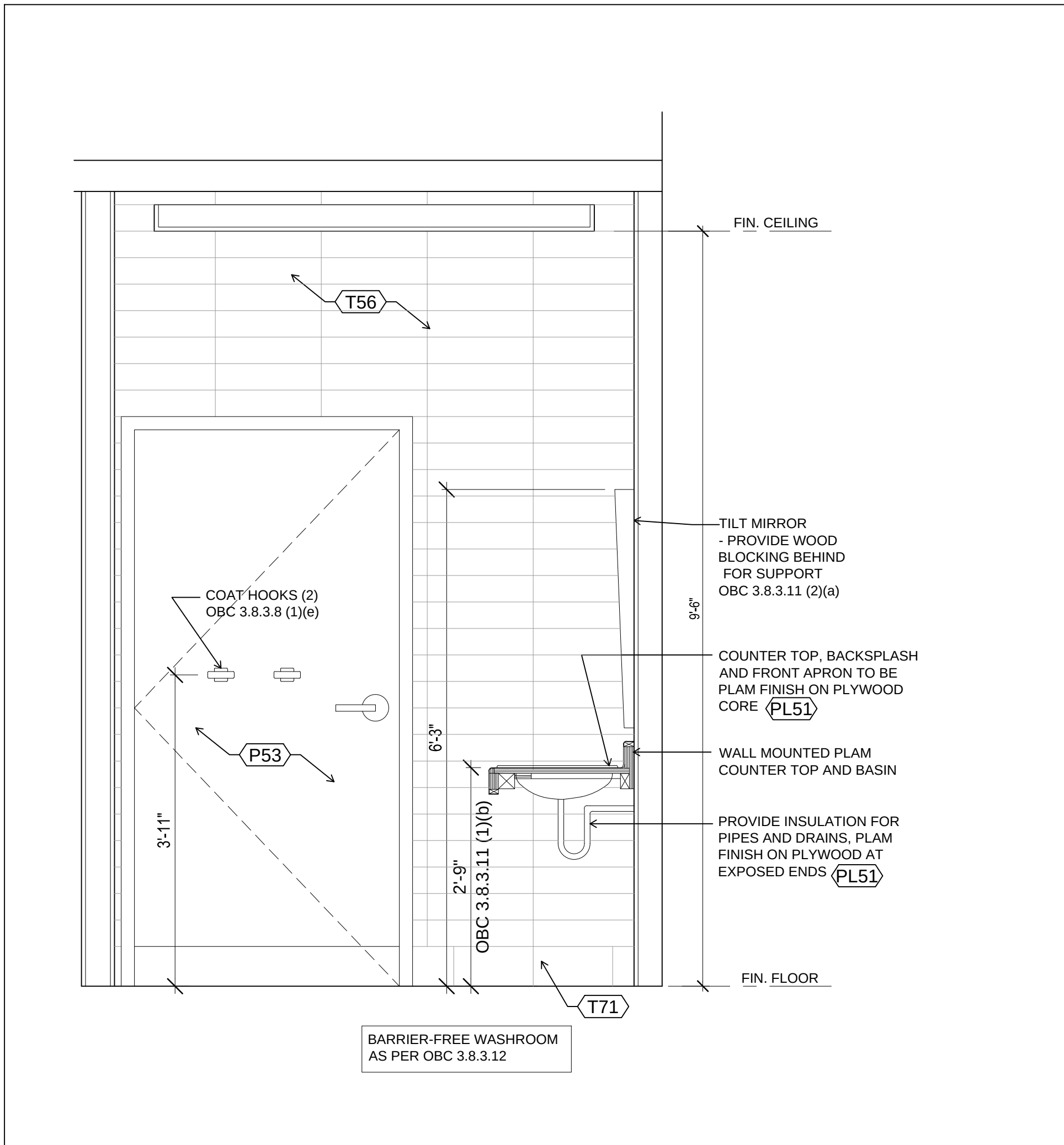
5 BARRIER-FREE WASHROOM - EAST ELEVATION SCALE: 3/4"=1'-0"
