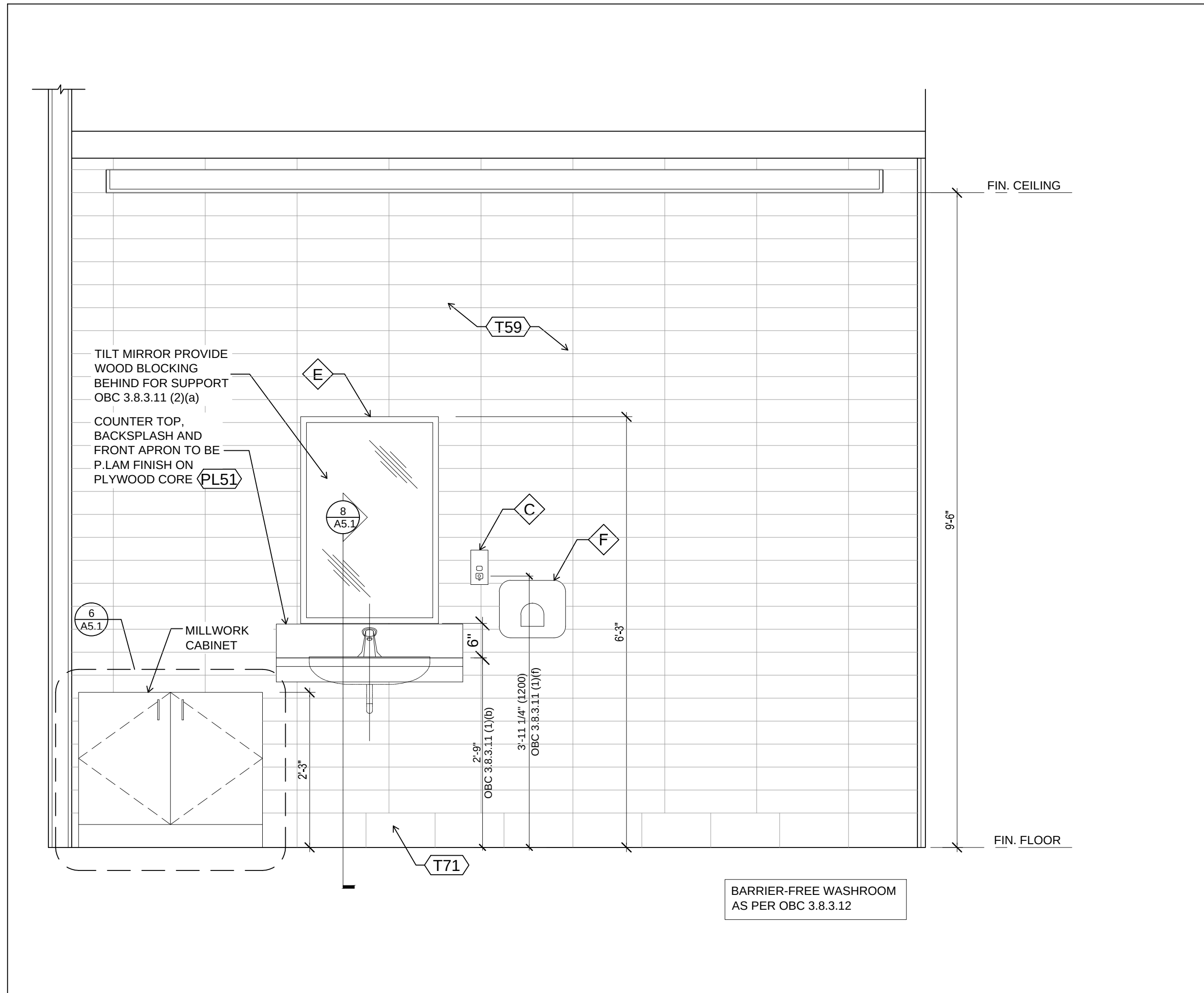
4 BARRIER-FREE WASHROOM - SOUTH ELEVATION SCALE: 3/4"=1'-0"
