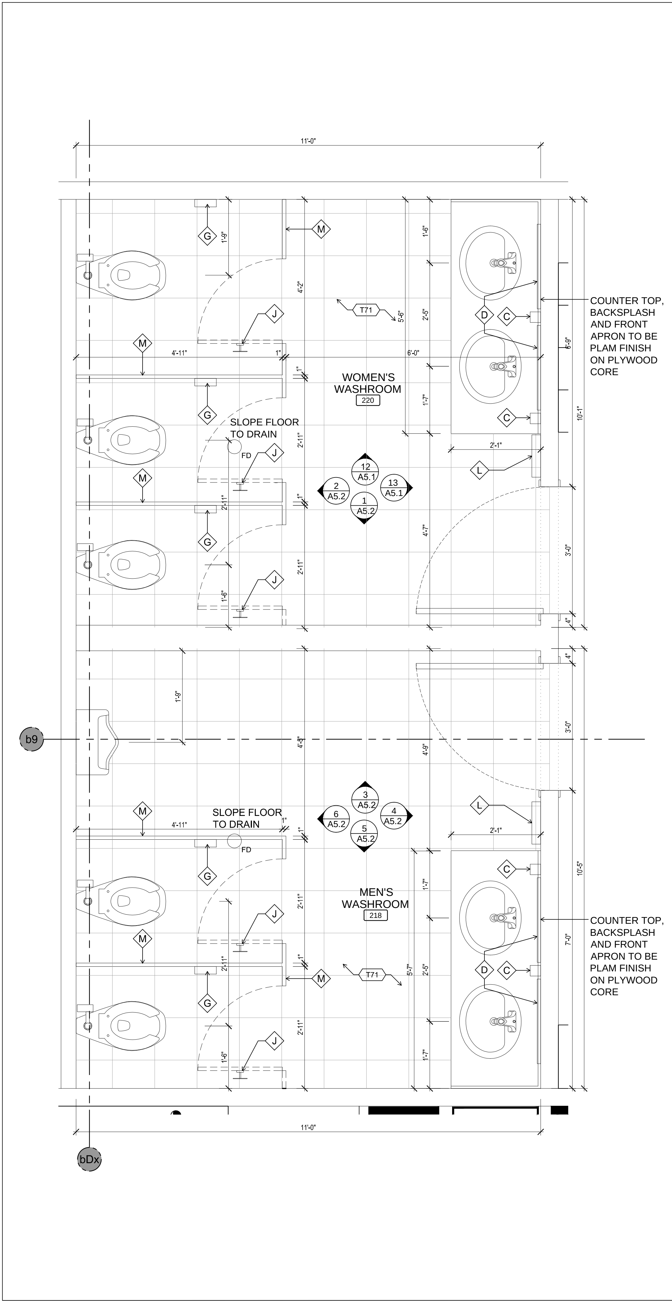
11 MENS AND WOMENS WASHROOM 204 & 205 SCALE: 3/4"=1'-0"
