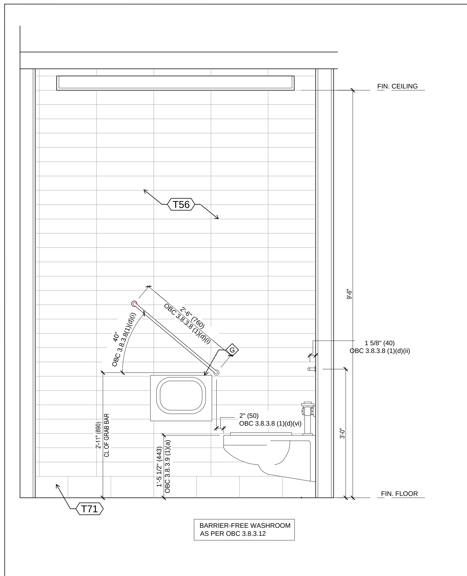
3 BARRIER-FREE WASHROOM - WEST ELEVATION SCALE: 3/4"=1'-0"
