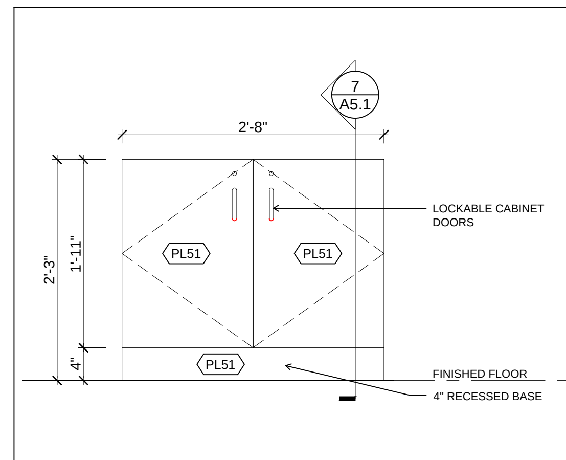
6 WASHROOM CABINET ELEVATION SCALE: 1/2"=1'-0"
